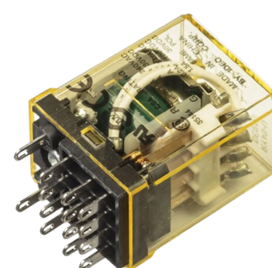
ULM20439 RELAY - 24V; 4 WECHS
