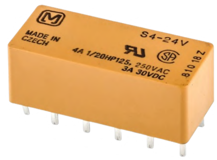
ULM20442 STEP RELAY - 24V; 2 WECHS
