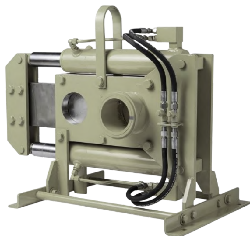
ULM20186 HYDRAULIC GATE VALVE – ZX125
