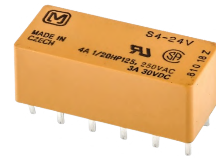
ULM20443 RELAY - 24V; 3/4A; 2S, 2Ö
